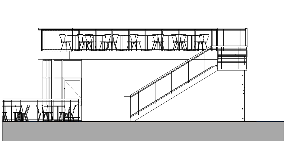
Elevation South 1 : 100
