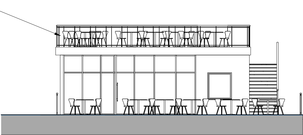
Elevation West 1 : 100
