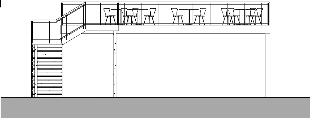
Elevation East 1 : 100
