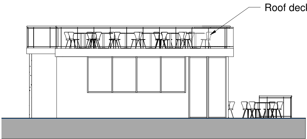
Elevation North 1 : 100
